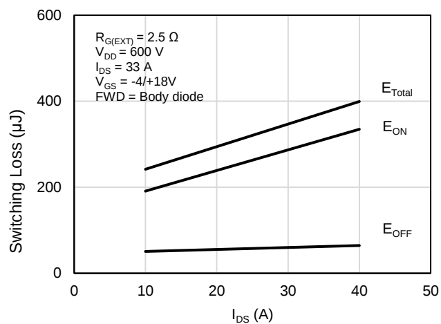
Figure 30: Clamped Inductive Switching Energy vs. I_{DS}
