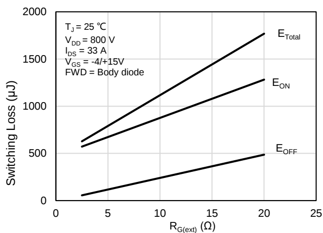
Figure 27: Clamped Inductive Switching Energy vs. R_{G(ext)}
