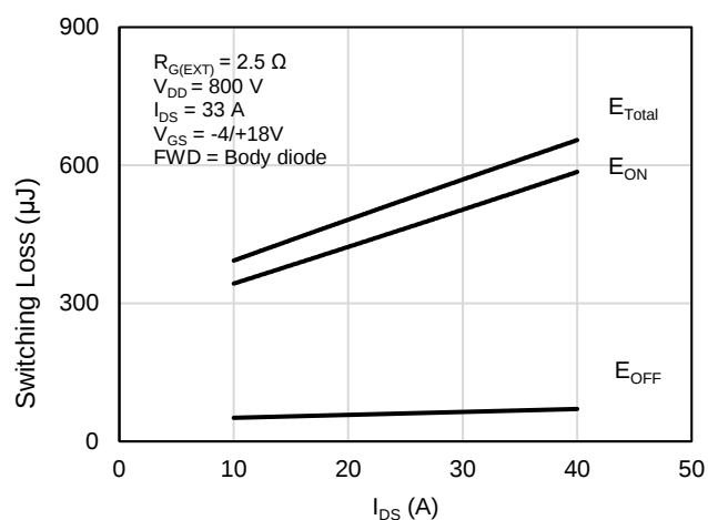
Figure 29: Clamped Inductive Switching Energy vs. I_{DS}
