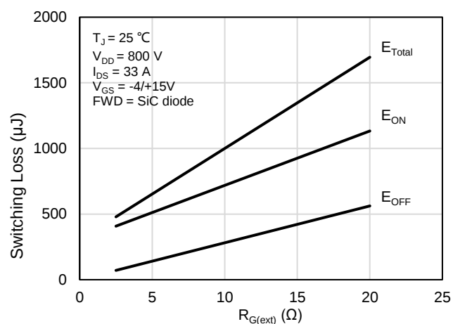
Figure 28: Clamped Inductive Switching Energy vs. R_{G(ext)}
