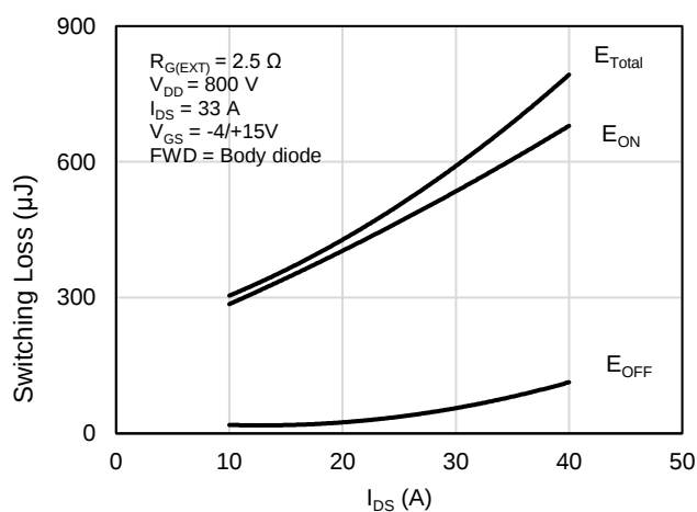
Figure 23: Clamped Inductive Switching Energy vs. I_{DS}
