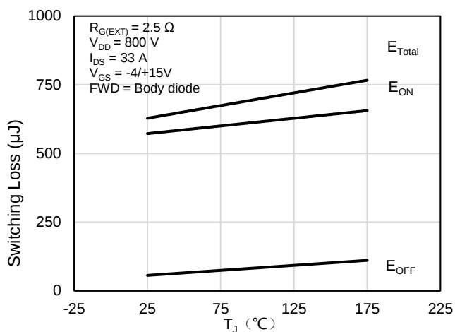
Figure 25: Clamped Inductive Switching Energy vs. T_j
