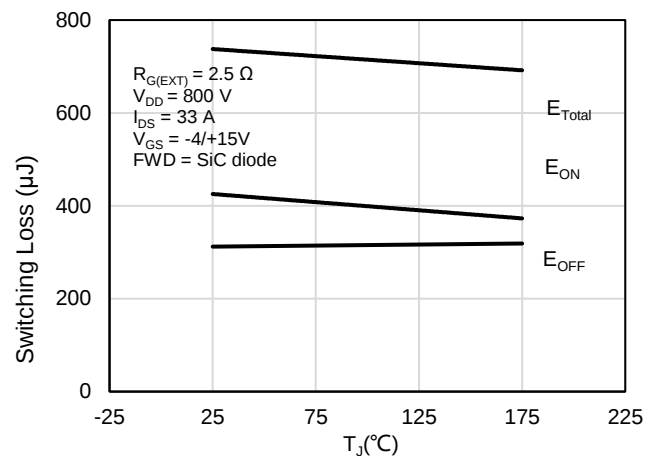
Figure 26: Clamped Inductive Switching Energy vs. T_j
