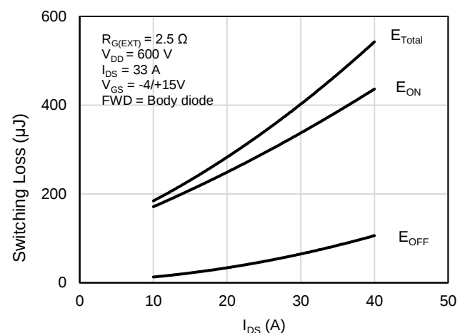
Figure 24: Clamped Inductive Switching Energy vs. I_{DS}
